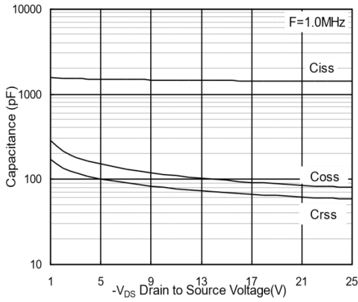
Fig.7 Capacitance
