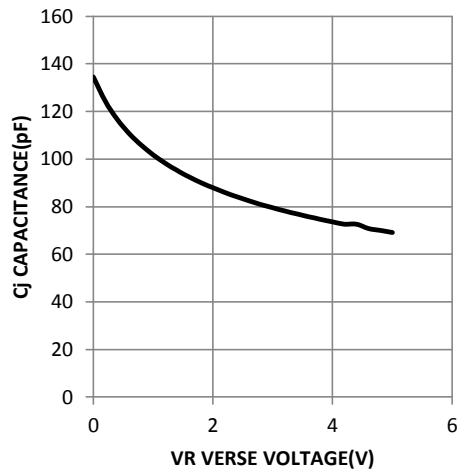
Fig 3. Capacitance character
