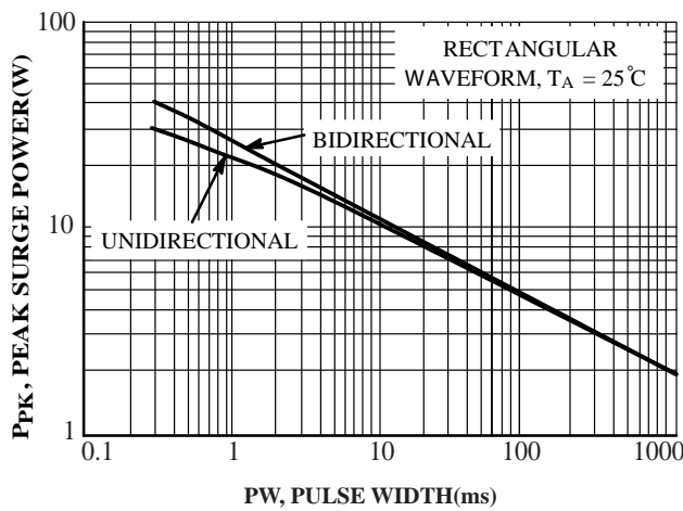
FIG.7 Maximum Non-repetitive Surge Power, P PK Versus PW
